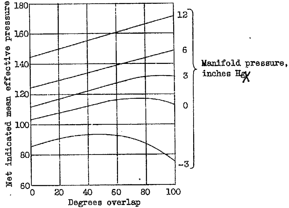
Fig.3 Variation of net indicated mean effective pressure with overlap
