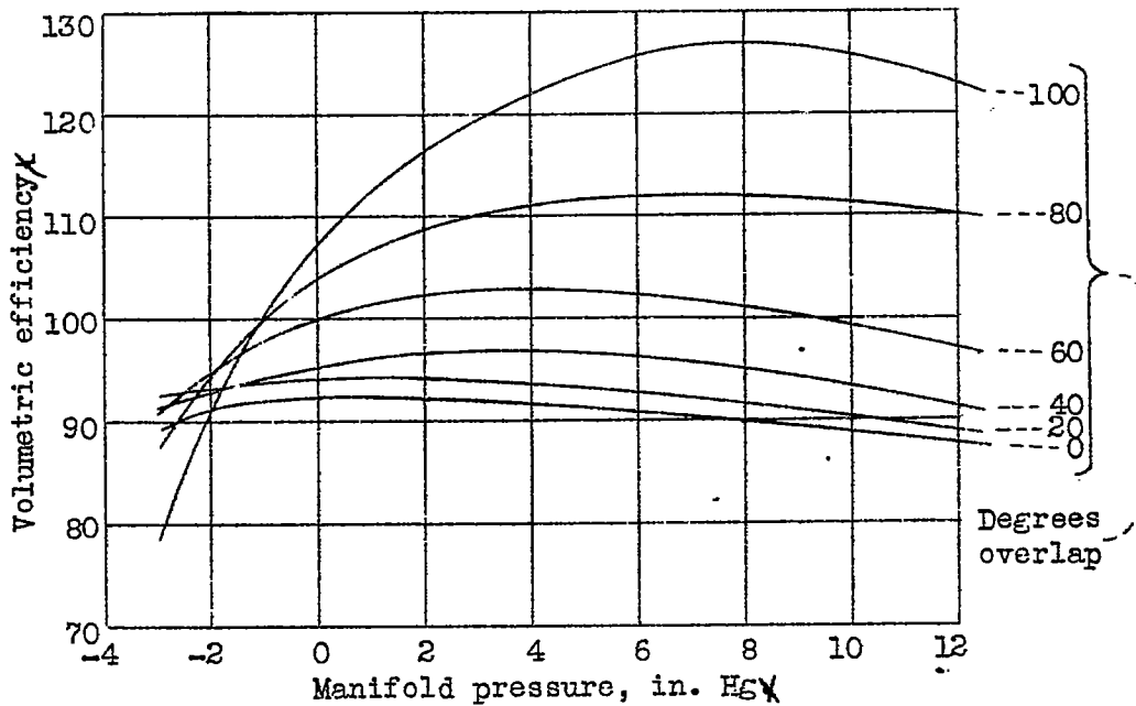
Fig. 8 Variation in volumetric efficiency with overlap efficiency based on air at intake pressure and temperature and corrected for compression of residual products
