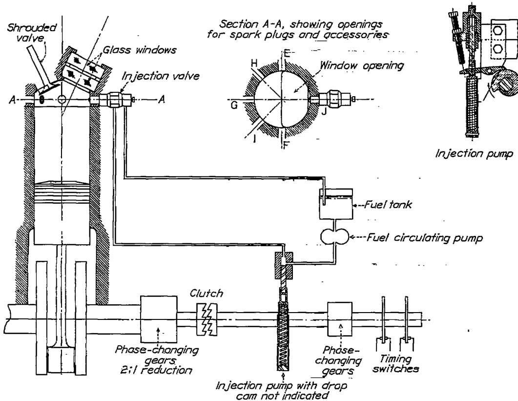
FIGURE 1.—Diagrammatic sketch of combustion apparatus.
