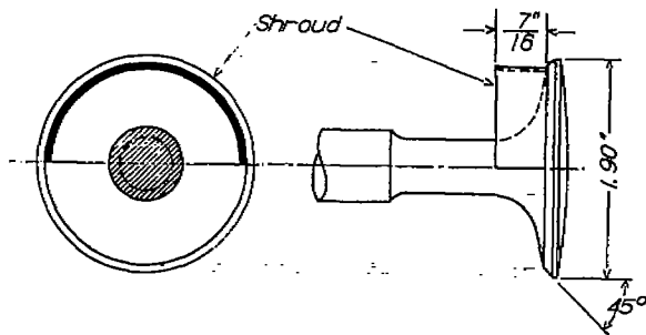
FIGURE 2.—Sketch of shrouded valve.
