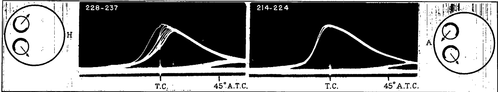
FIGURE 10.—Effect of gas movement on cycle reproducibility. Engine speed, 600 r. p. m.; one spark plug.
