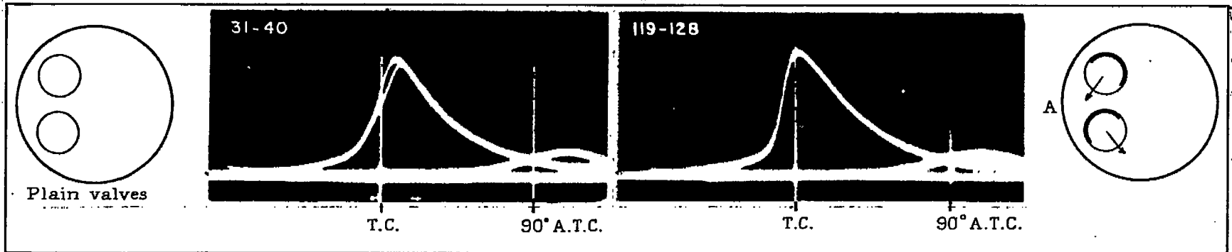
FIGURE 11.—Comparison of effects on cycle reproducibility of plain valves and of shrouded valves set for full axial swirl. Engine speed, 1,000 r. p. m.; two spark plugs.
