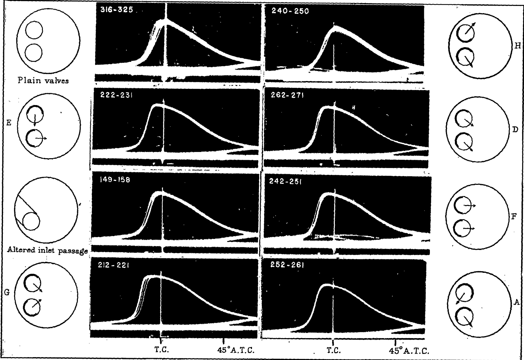
FIGURE 9.—Effect of gas movement on cycle reproducibility. Engine speed, 600 r. p. m.; two spark plugs.
