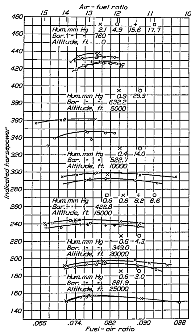
FIGURE 2.—Altitude chamber tests
